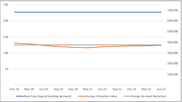
INCUBATOR BUILDING EUI**
